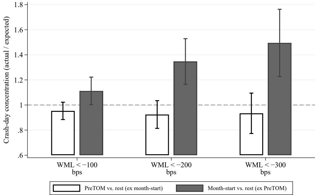
Figure 5: Crash-day concentration by calendar window. Each point plots the ratio of actual crash-day share to calendar share; whiskers show 95% confidence intervals. The dashed horizontal line marks a ratio of one, the value expected if crash days were distributed uniformly across the calendar. Daily WML returns are value-weighted. Momentum deciles use NYSE breakpoints applied to all NYSE, AMEX, and NASDAQ stocks in CRSP; assignments are held constant within each calendar month. Sample: 1980–2025.
