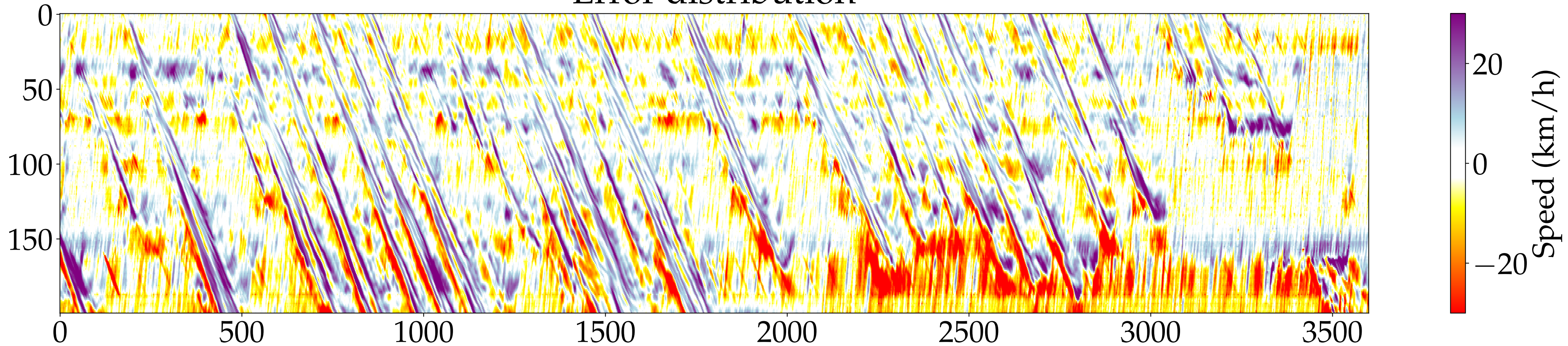
Error distribution
