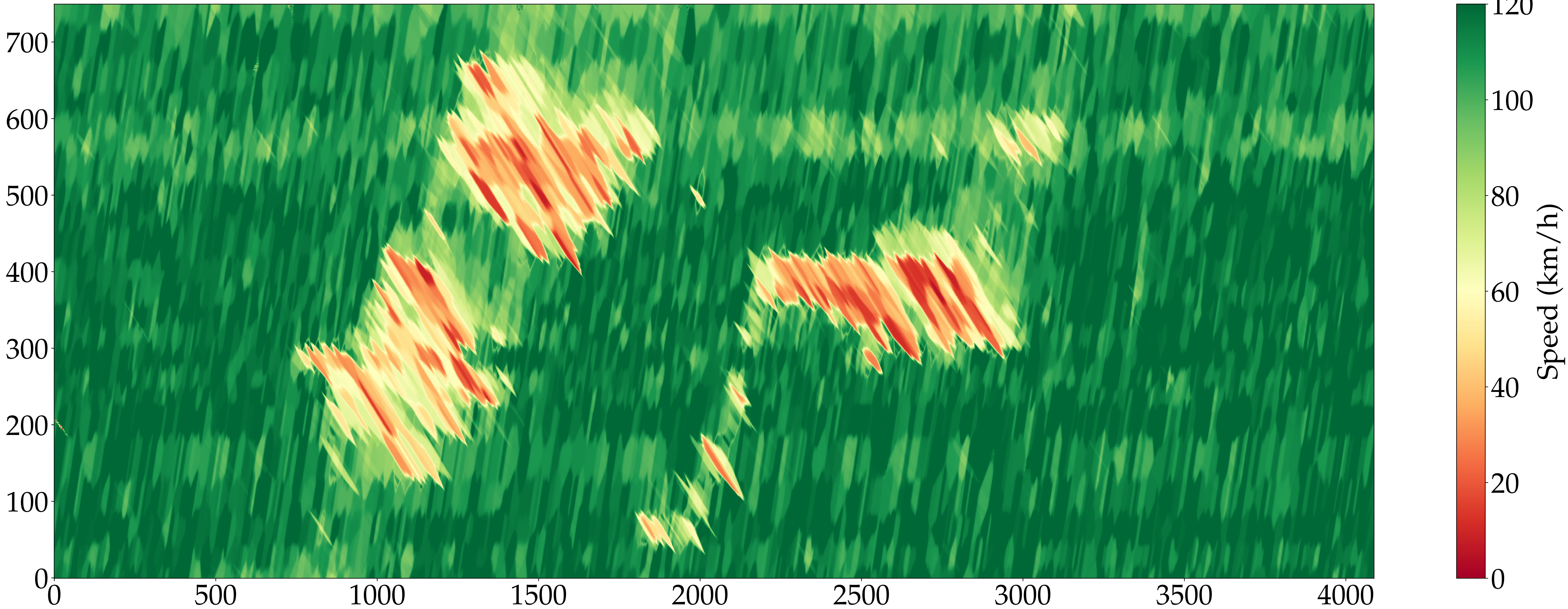
Interstate 95 Corridor reconstruction with ASM
