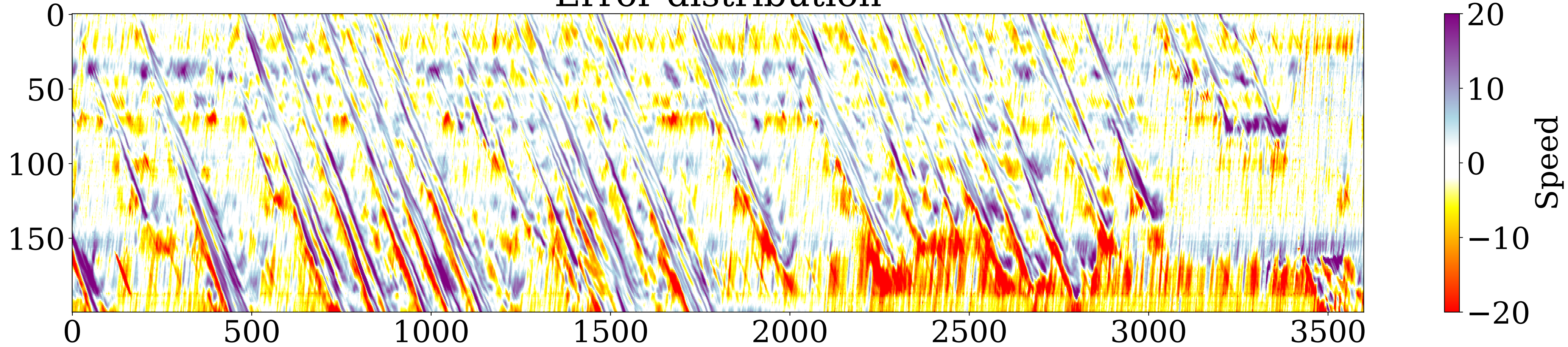
Error distribution
