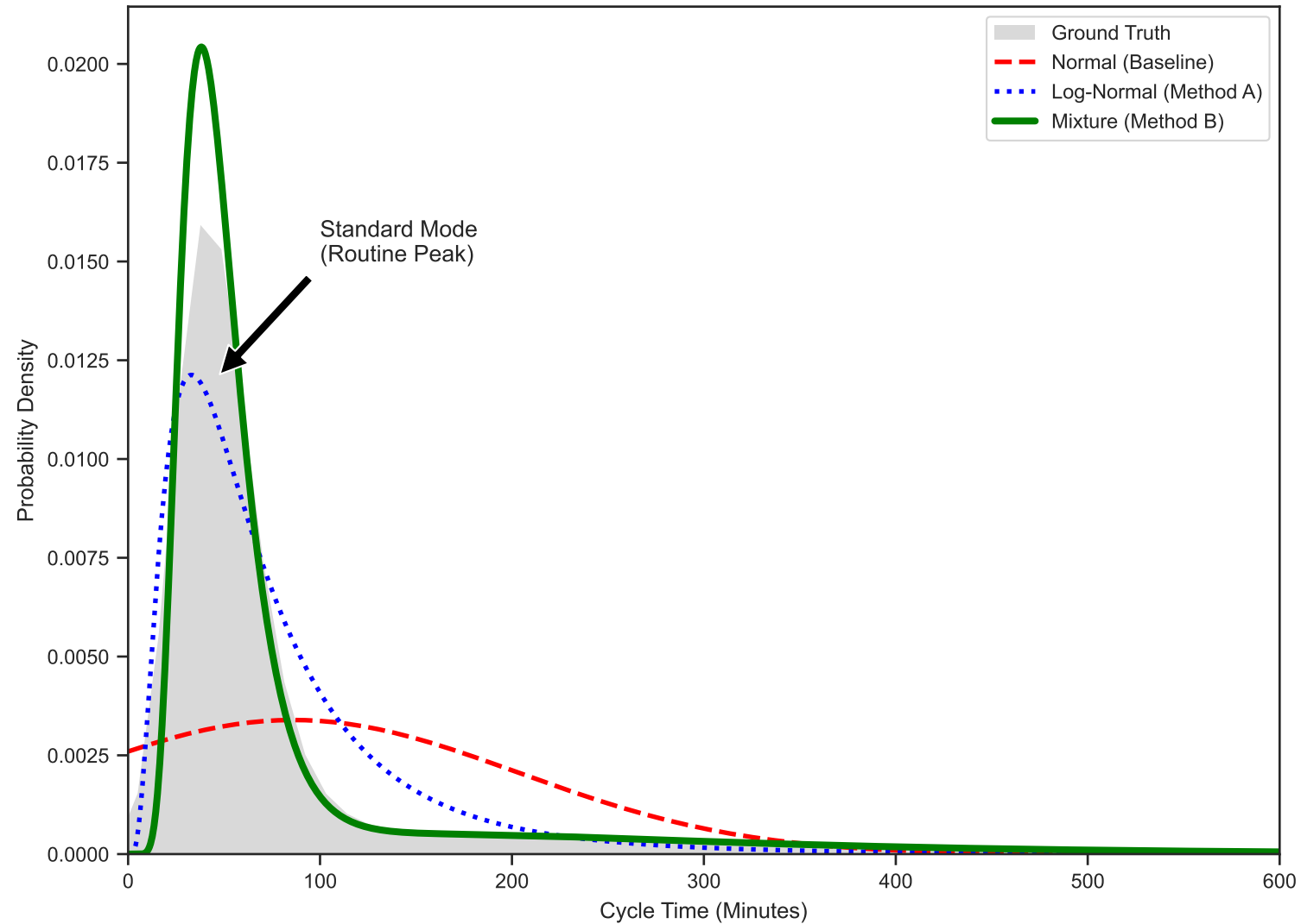
Fig 1a: Overall Distribution Fit (Macro View)
