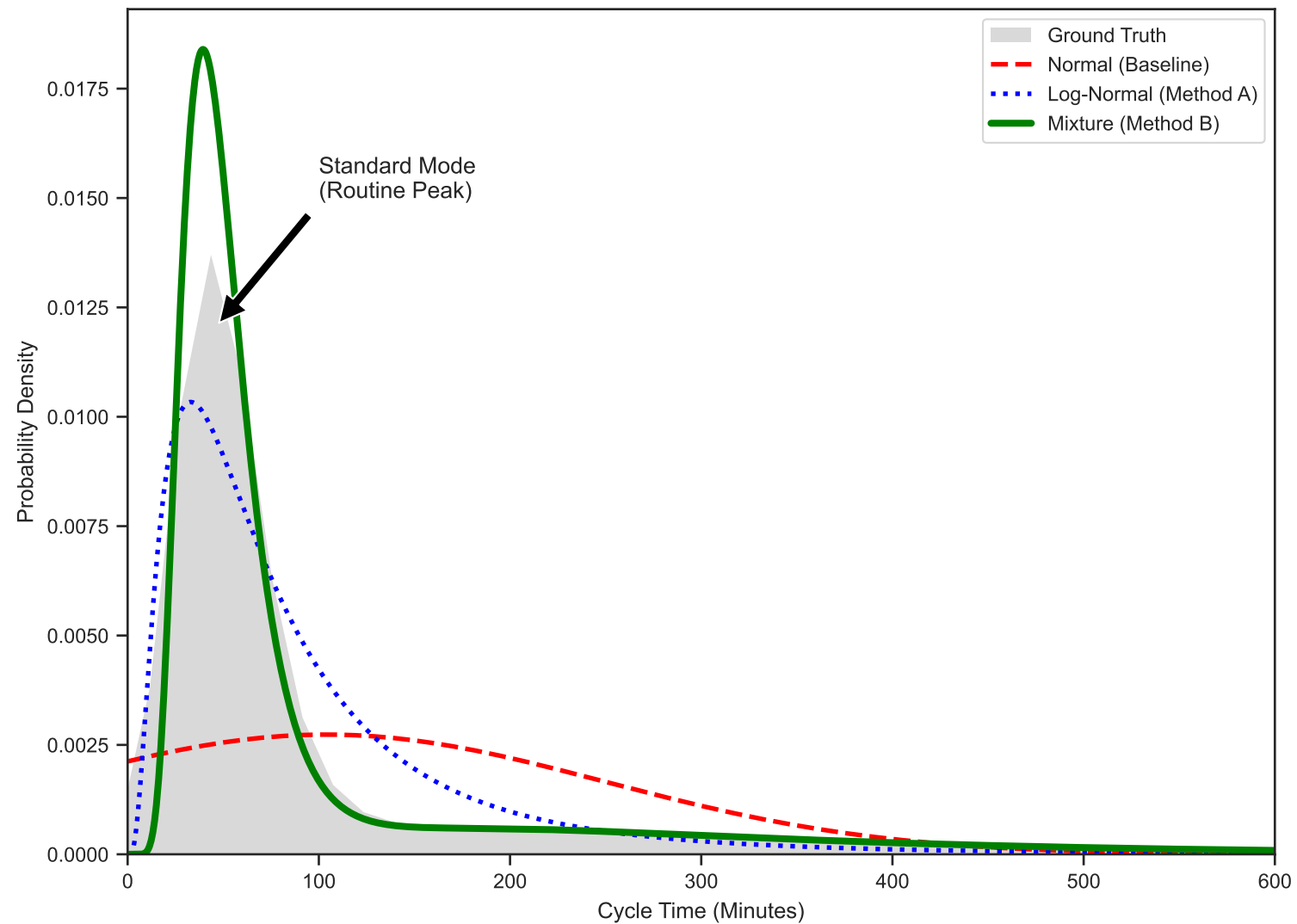
Overall Distribution Fit (Macro View)
