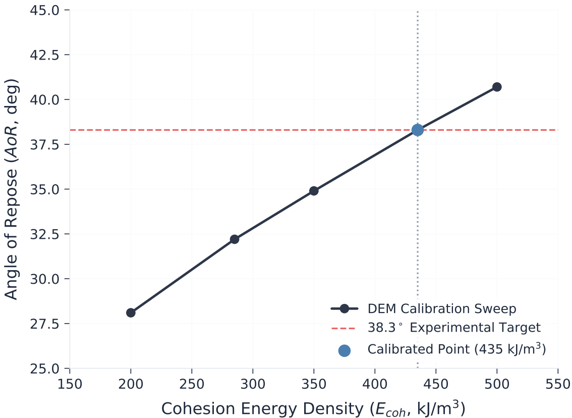
Measured Repose Angle vs Cohesion Energy Density
