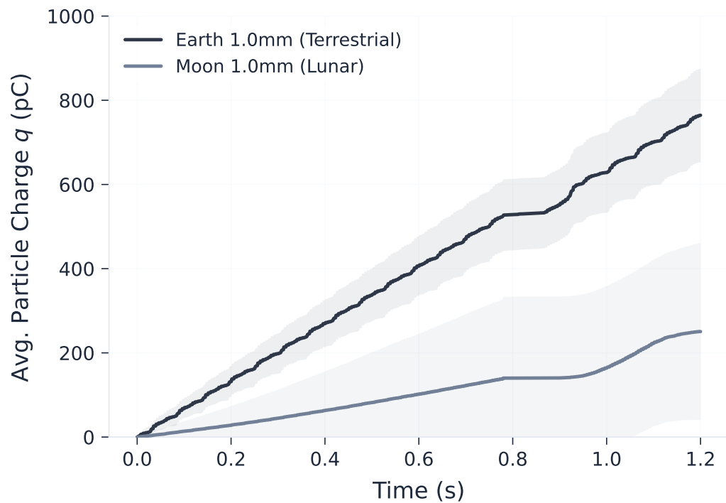
(b) Charge Accumulation History
