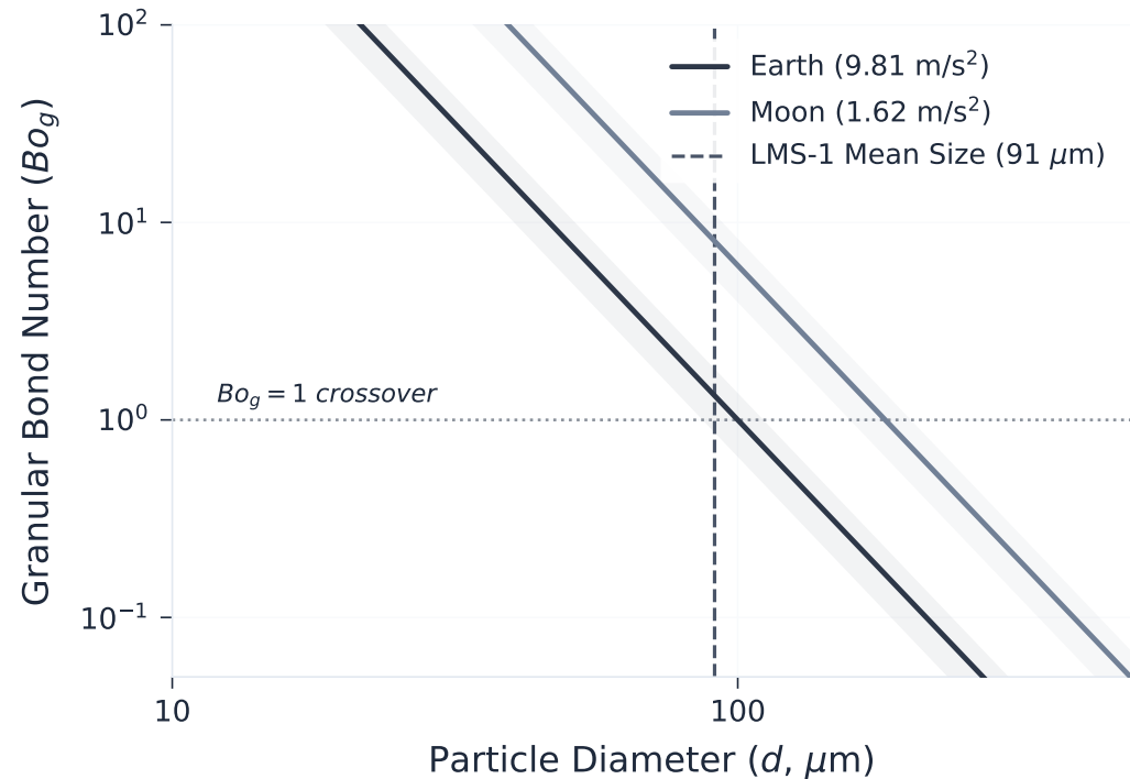
(a) Analytical Granular Bond Number
