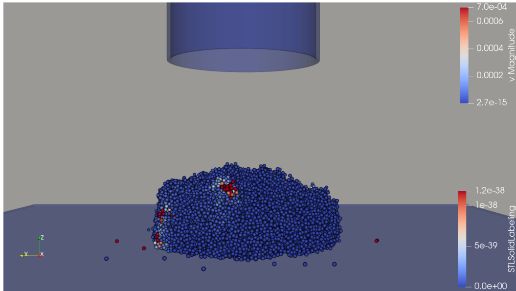
(a) 3D Conical Heap Render (20k Particles)
