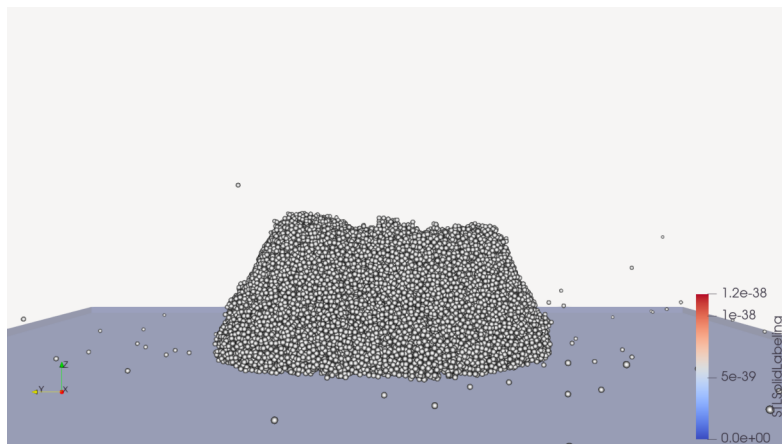
(c) 5k Conical Heap (ParaView)
