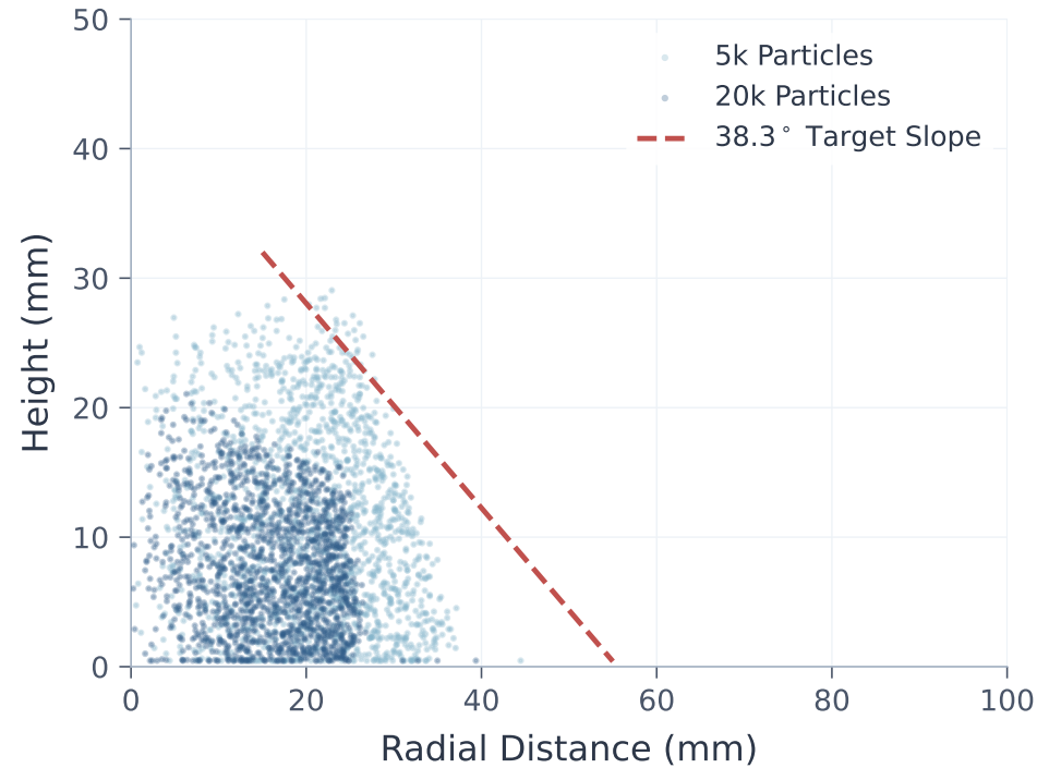
(a) Scale Convergence Profile
