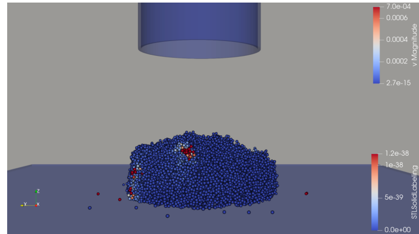
(c) Settled 3D Heap (ParaView)
