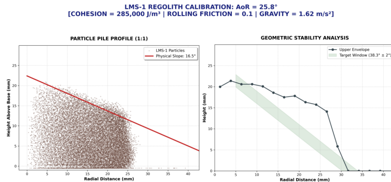
(b) Fitted Slope Profile (20k)
