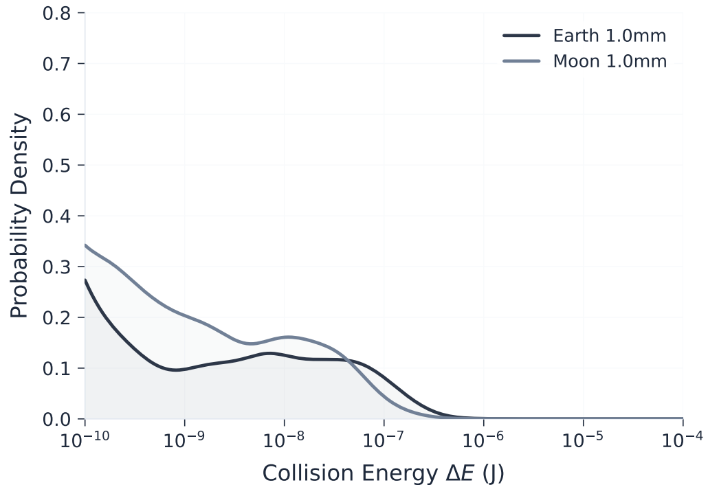
(b) Collision Energy Distribution
