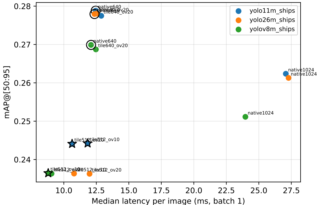
Accuracy-latency Pareto (SHIPS)
