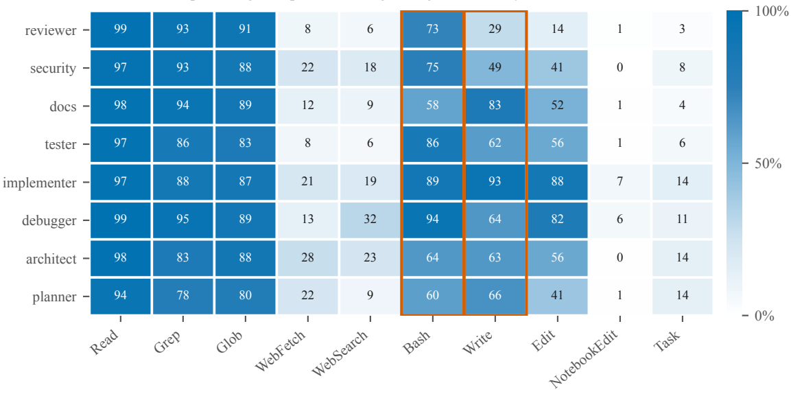
percentage of specifications granting each tool, by declared role
