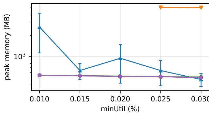
C8T1S5I8N5K
