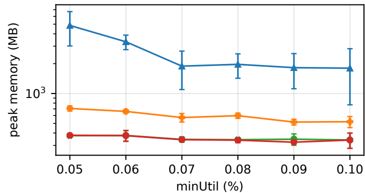
KOSARAK
