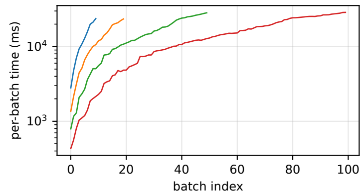
C8T1S5I8N5K
