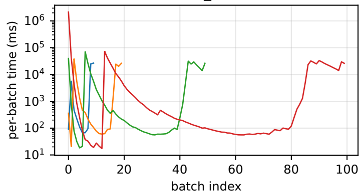
LEVIATHAN
