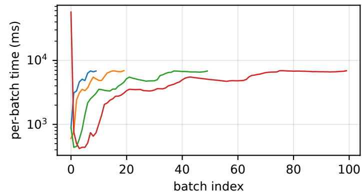
KOSARAK
