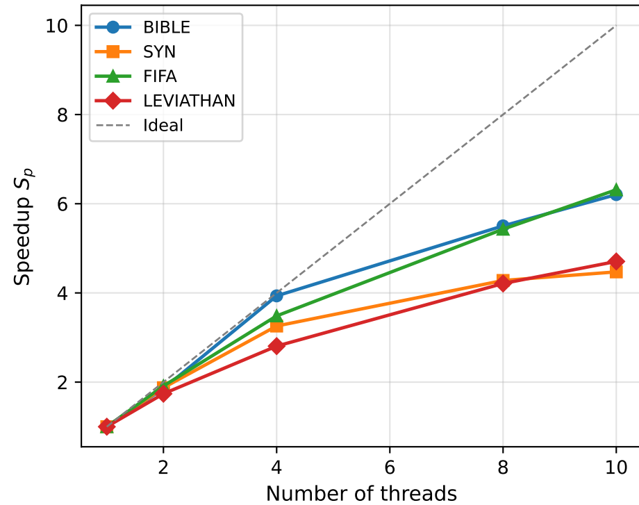
(a) Mining speedup vs. threads
