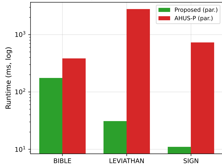
(c) Proposed vs. AHUS-P (T=10)
