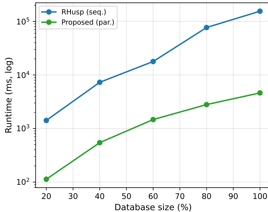
(b) Data scaling — KOSARAK
