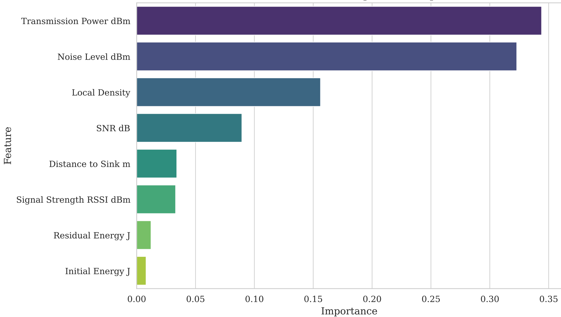
XGBoost Global Feature Importance (Split-Based)
