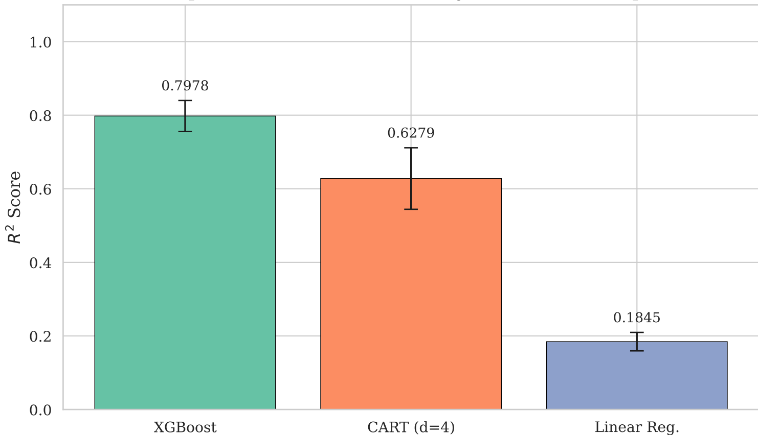
Model Comparison: Predictive Accuracy ( R^2 , 5-Fold GroupKFold CV)
