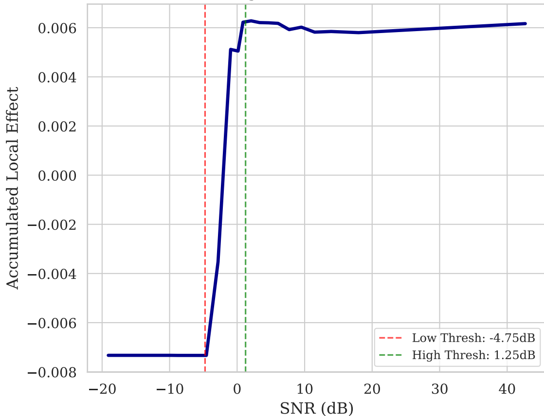
(a) ALE: Signal-to-Noise Ratio (SNR)
