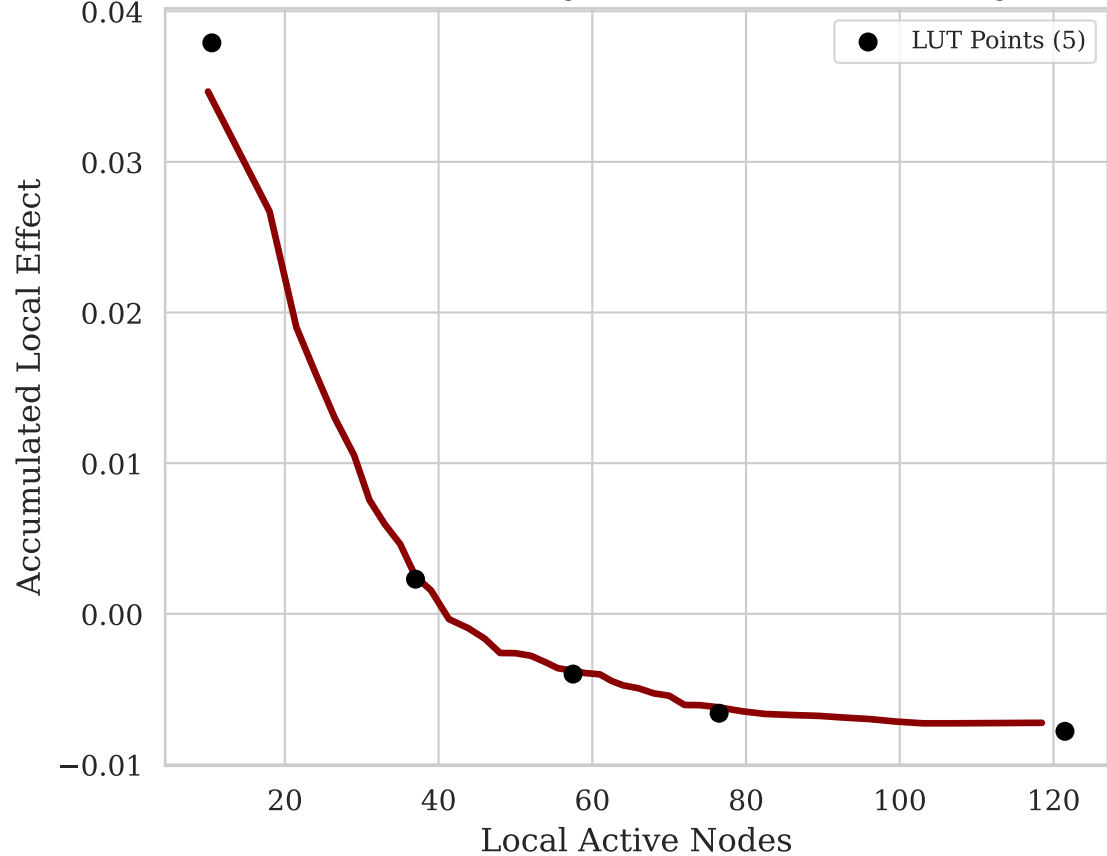
(b) ALE: MAC-Layer Contention (Density)
