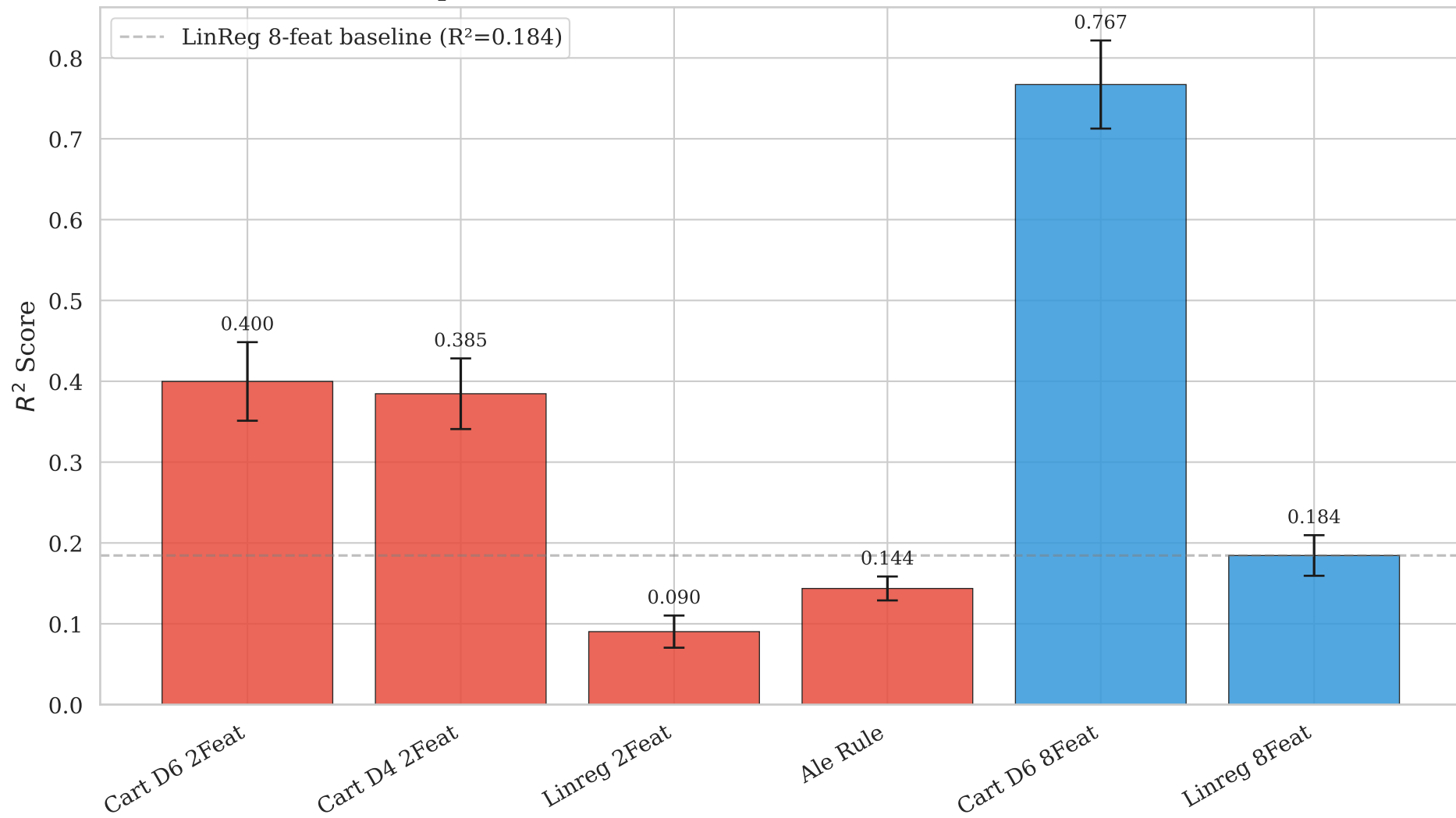
Fair Comparison: ALE Rule vs. Models with Same Feature Count
