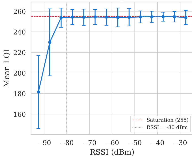
(b) LQI vs RSSI (per 5 dB bin)
