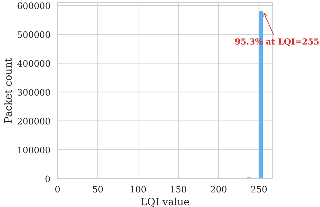
(a) LQI Distribution (AT86RF231)
