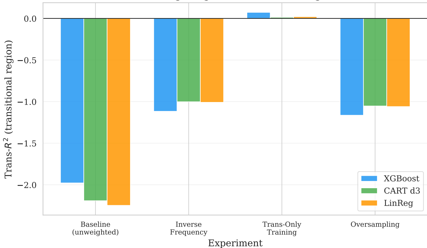
Effect of Class Reweighting on Transitional-Region Performance
