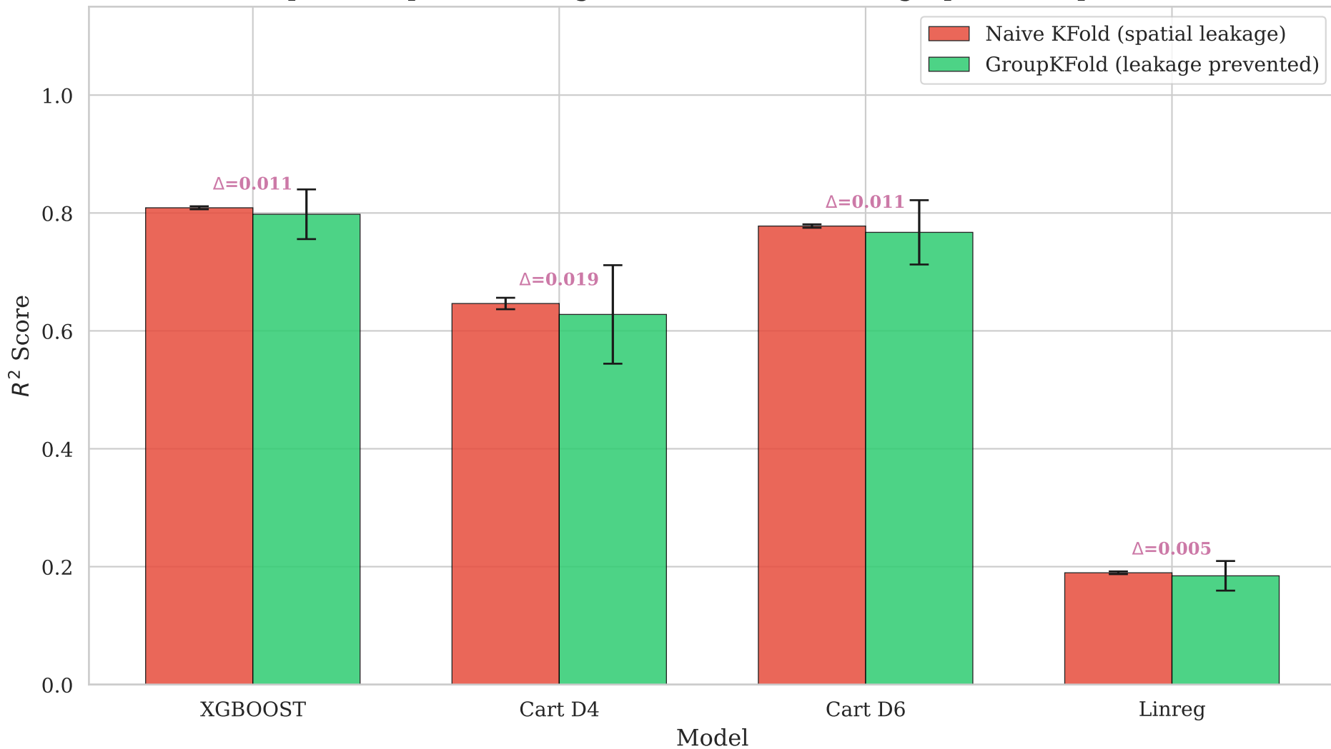
Impact of Spatial Leakage: Naive KFold vs. Geographic GroupKFold
