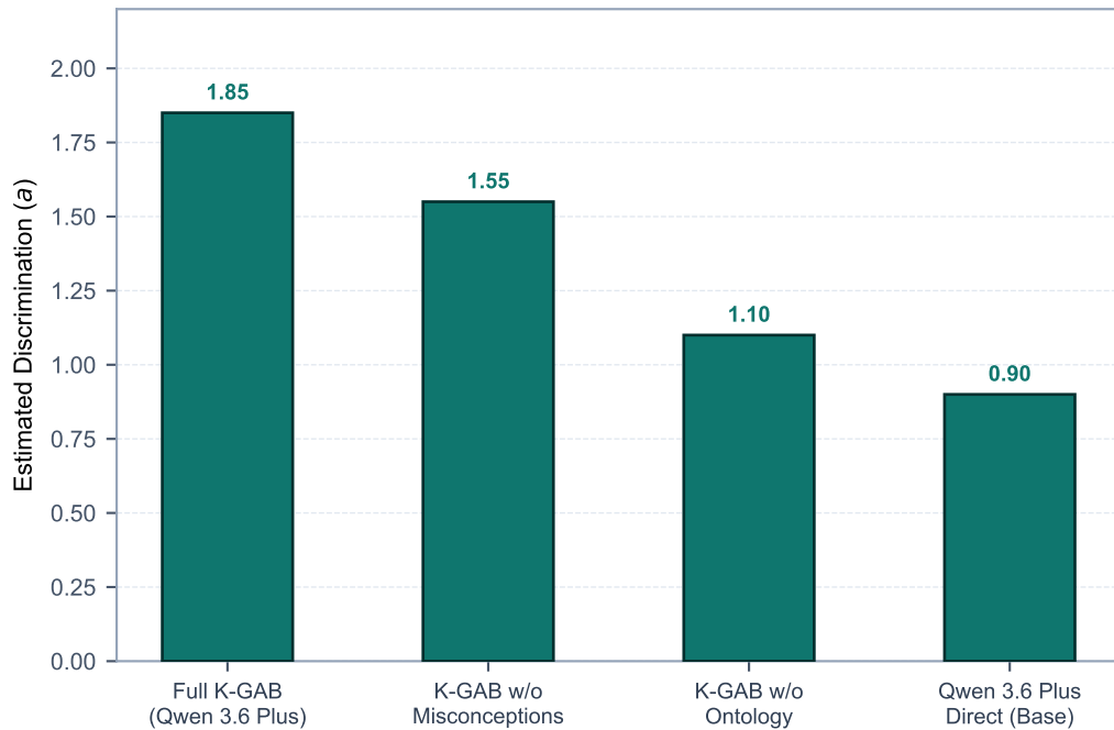
Panel A: Item Discrimination (a)
