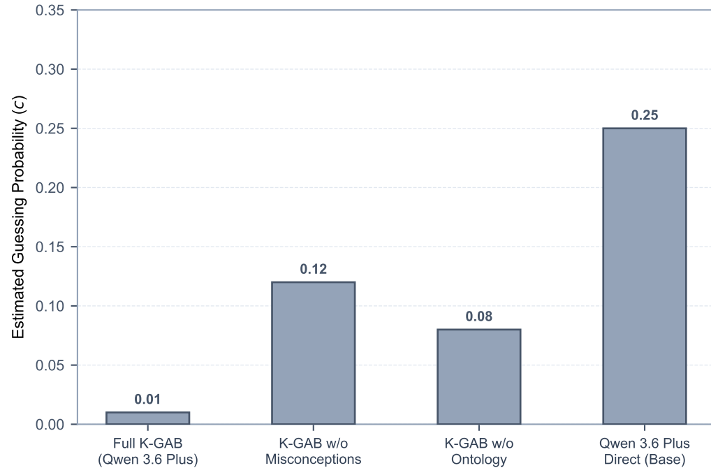
Panel B: Parameter Guessing (c)
