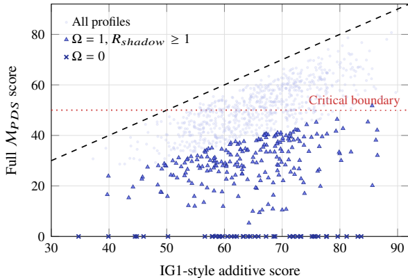
(a) Paired score divergence on the same 1,000 profiles
