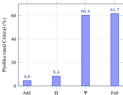
(b) Component ablation
