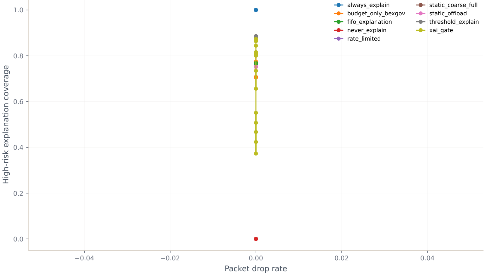
Budget frontier under adversarial explanation demand
