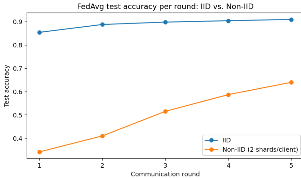
Figure: FedAvg test accuracy per communication round, IID vs. Non-IID.
