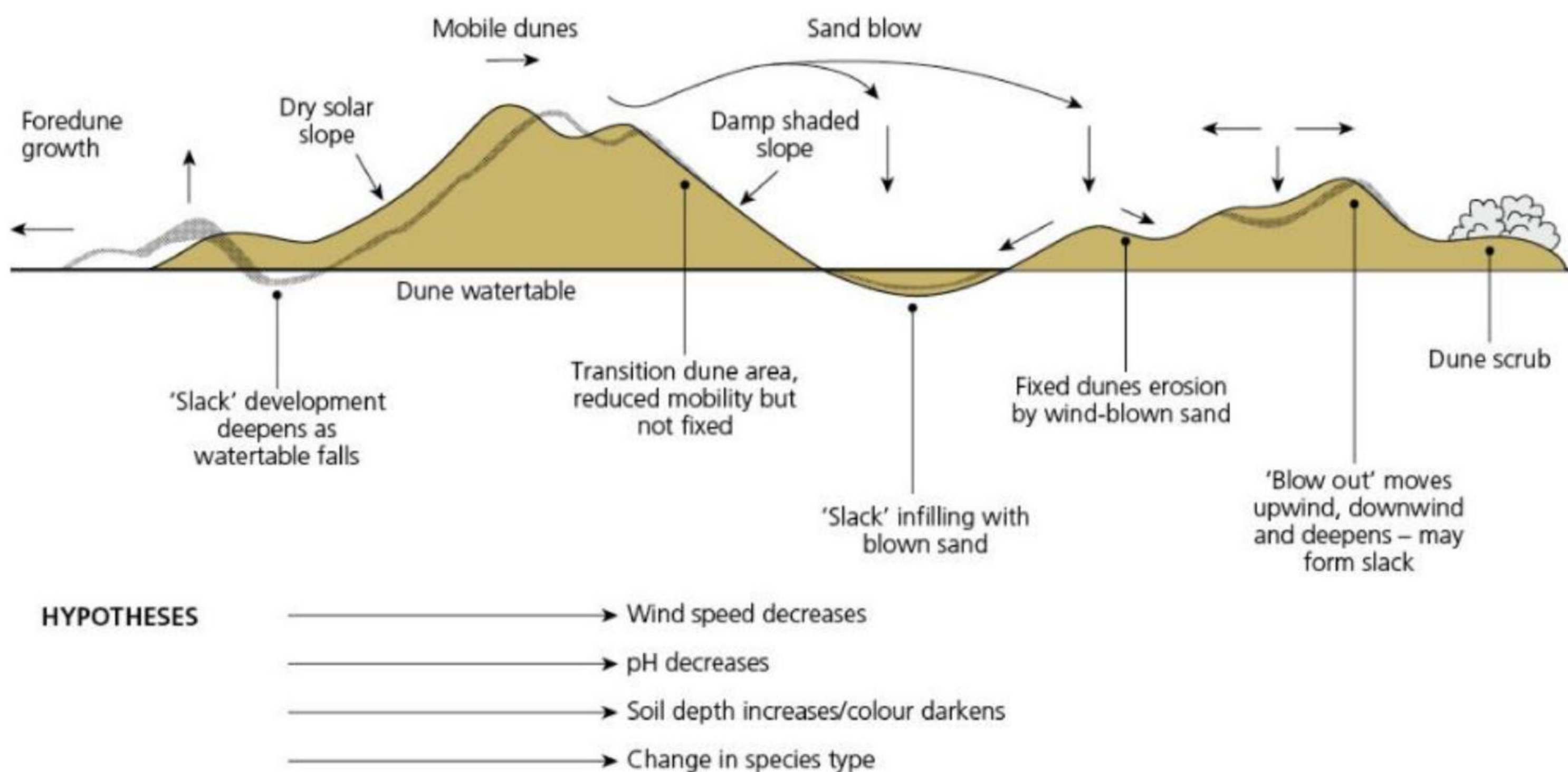
▲ Figure 2.41 The dynamic sand dune environment
