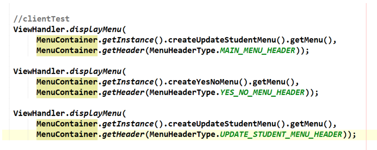
Figure 20: Using singleton pattern for menu, avoiding trash menu - Get Menu
