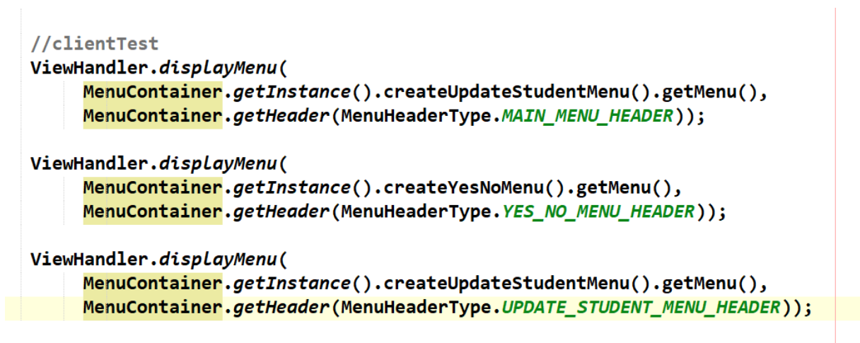
Figure 18: Using singleton pattern for menu, avoiding trash menu - Get Menu
