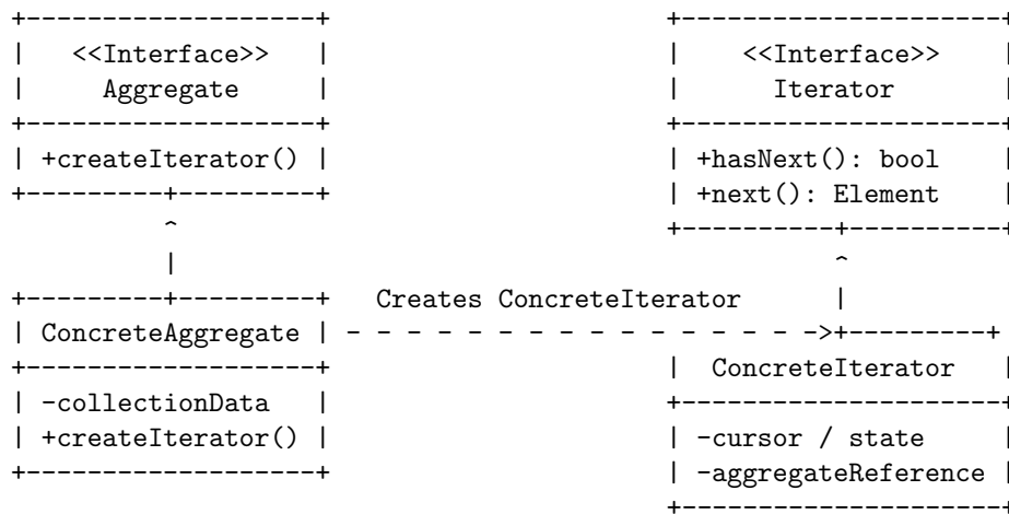
Figure 2.2: Iterator Pattern Architecture
