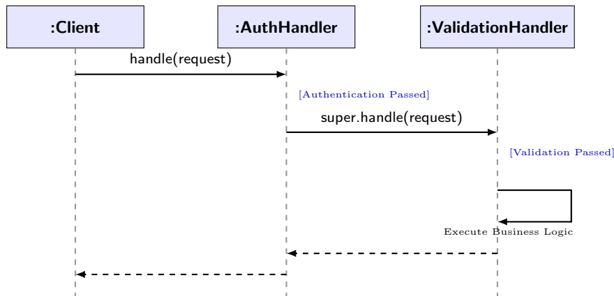
Figure 2.2: UML Sequence Diagram showing successful request execution flow
