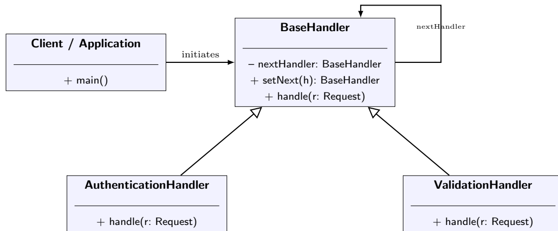
Figure 2.1: UML Class Diagram for Chain of Responsibility Pattern
