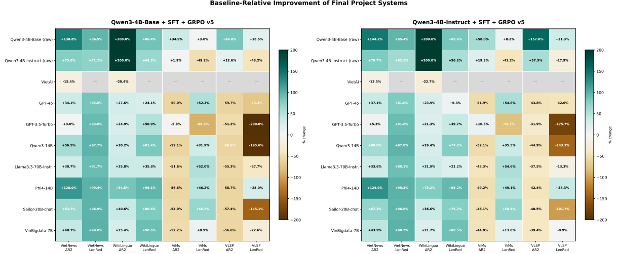
Figure 2: Baseline-relative improvement summary for the two final project systems. Each dataset is shown explicitly as a two-column block: positive \Delta R_2 means higher ROUGE-2, positive LenRed means smaller absolute summary length distance, and gray cells mark unavailable values. The first two rows are raw Qwen3-4B baselines, followed by external baselines. Cell text shows the exact percentage change, while color intensity is clipped for readability.
