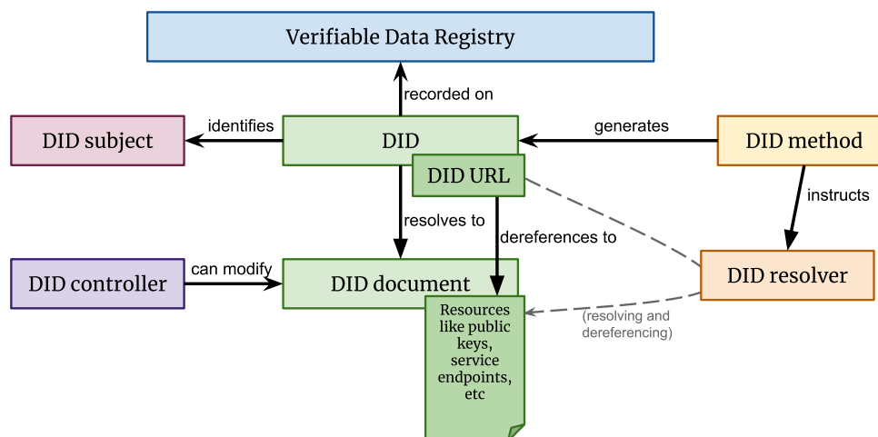
Figure 1 The basic components of DID architecture.
