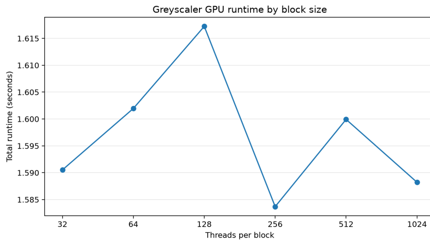
Figure 1: Total greyscale runtime for each GPU block size. Each point is one run.
