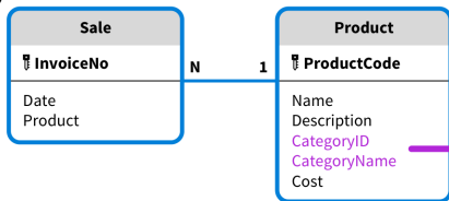
Alternative Data Models for the Same Data Set
