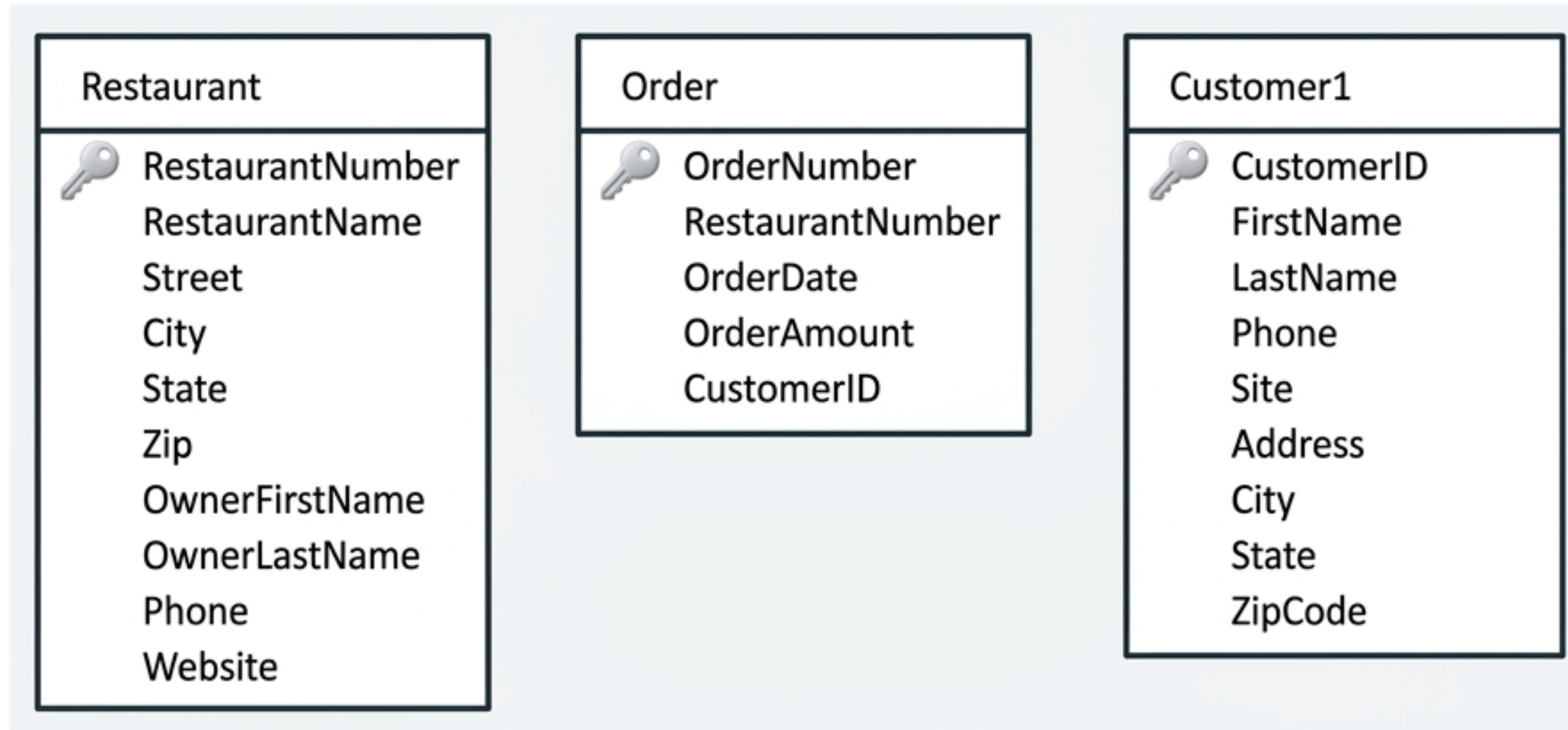
Restaurant, Order, Customer1 Database Schema
