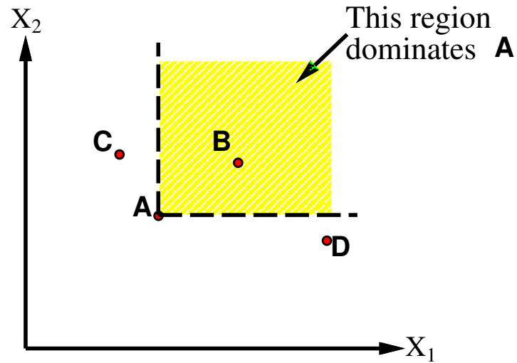
Deterministic attributes
