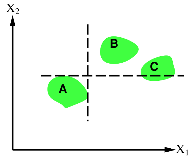
Uncertain attributes
