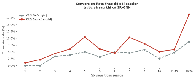
Fig. 4: Conversion rate by session length before and after SR-GNN intervention. X-axis: number of views per session; Y-axis: CR (%). Dashed line: baseline (before intervention).
