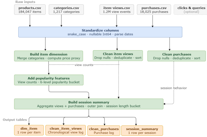
Fig. 1: Data preprocessing pipeline
