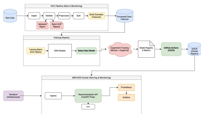
Fig. 11: End-to-end pipeline: from raw interactions to production serving via DVC, MLflow, FastAPI, and Kubernetes.
