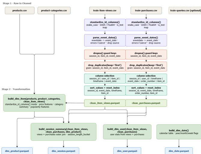
Fig. 1: Data preprocessing pipeline
