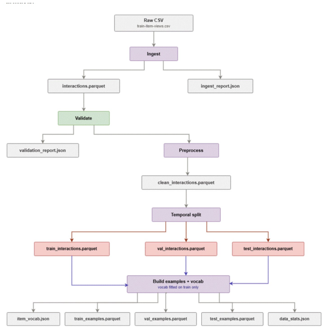
Fig. 9: Data pipeline flowchart - end-to-end flow from raw CSV to split examples and vocabulary for training SRGNN model.
