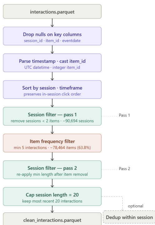
Fig. 10: Detailed preprocessing flow, from interactions.parquet to clean_interactions.parquet.
