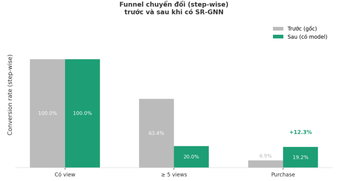
Fig. 5: Step-wise conversion funnel before and after SR-GNN intervention.
