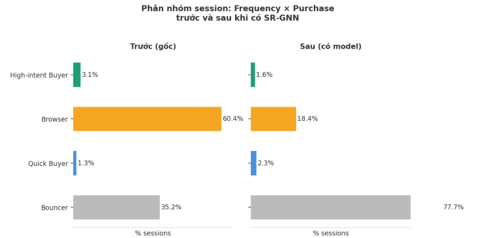
Fig. 6: Session segmentation by interaction frequency and purchase outcome, before (left) and after (right) SR-GNN intervention. Frequency threshold: 5 views.
