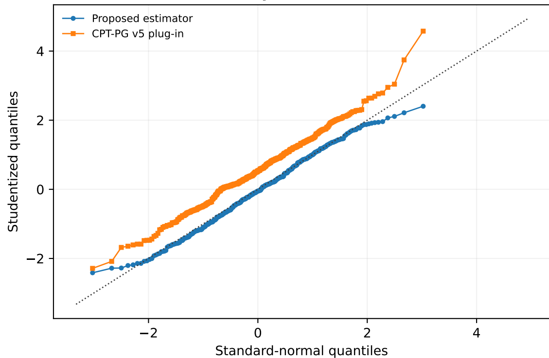
C Studentized normality
