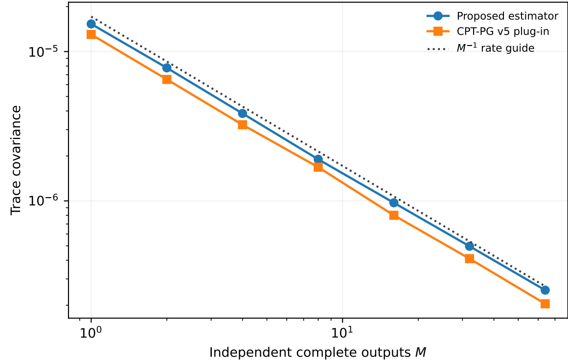
B Variance and M^{-1} scaling
