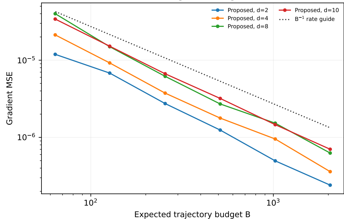
D Fixed-dimensional budget scaling
