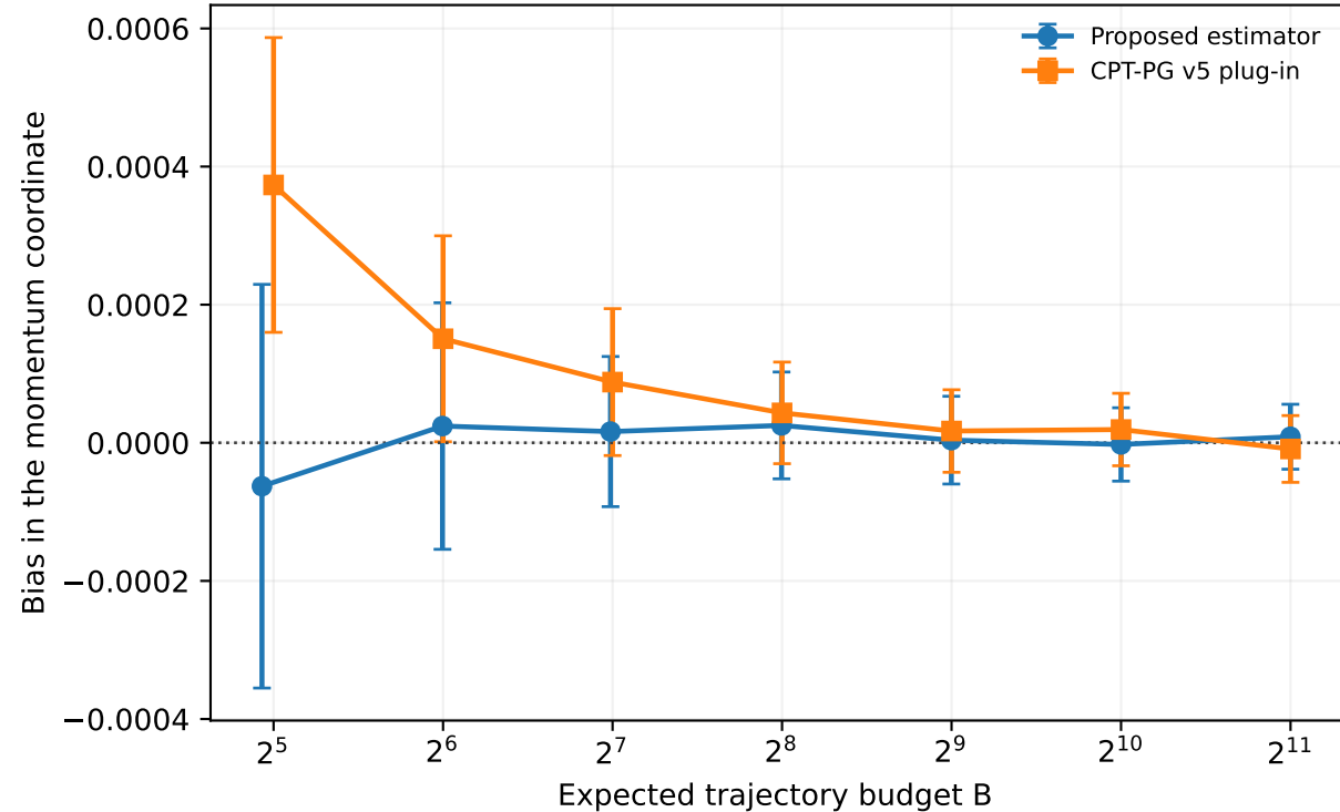
A Finite-sample bias
