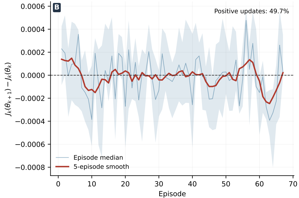
Paired same-episode update gain
