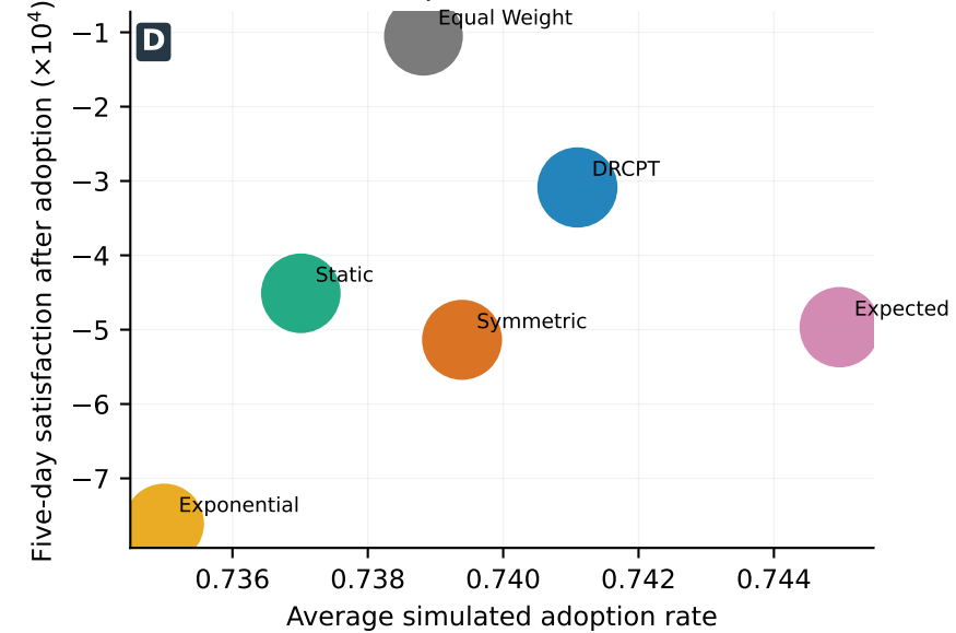
Method-level adoption--satisfaction trade-off
