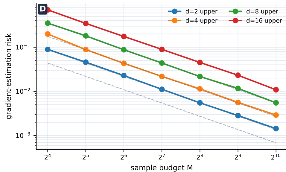
Minimax scaling: d/M
