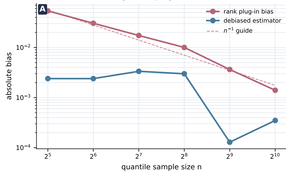
Bias diagnostic: plug-in vs debiased
