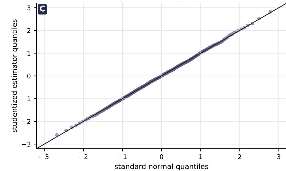
Asymptotic normality diagnostic
