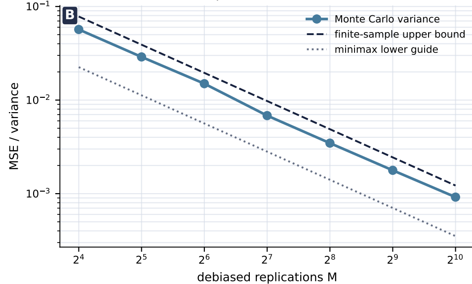
Finite-sample variance and M^{-1} rate
