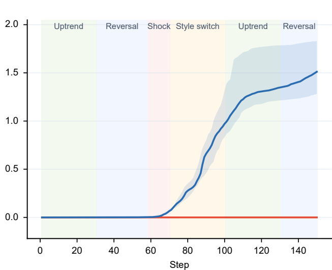
Dynamic local regret
