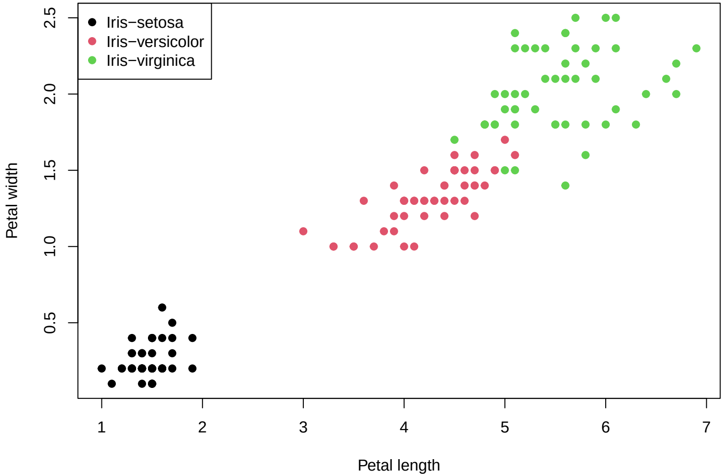
Plot of dependencies of petal length and width
