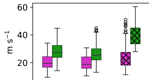
Max. 0-6 km bulk shear
