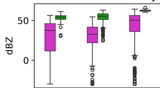
Max. radar reflectivity
