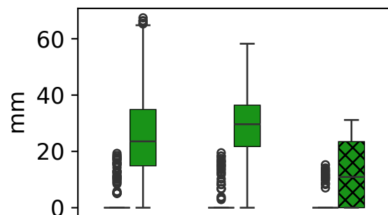
Max. hail diameter
