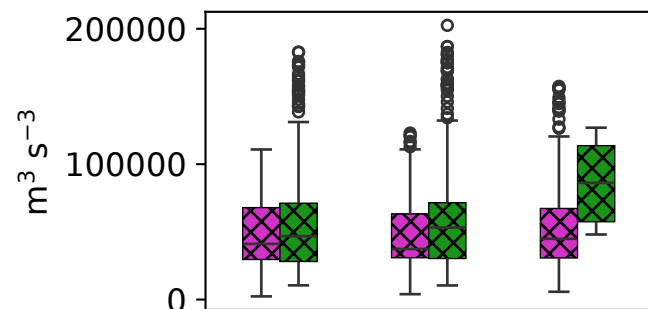
CAPE x shear
