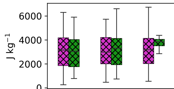
Max. CAPE
